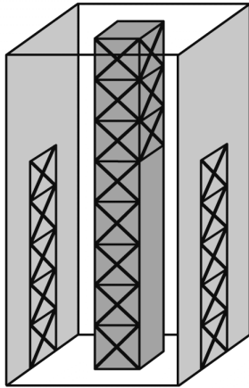
2 Figure 6.2 Illustration of lateral system with bracing elements repositioned over 3 height of the structure.
