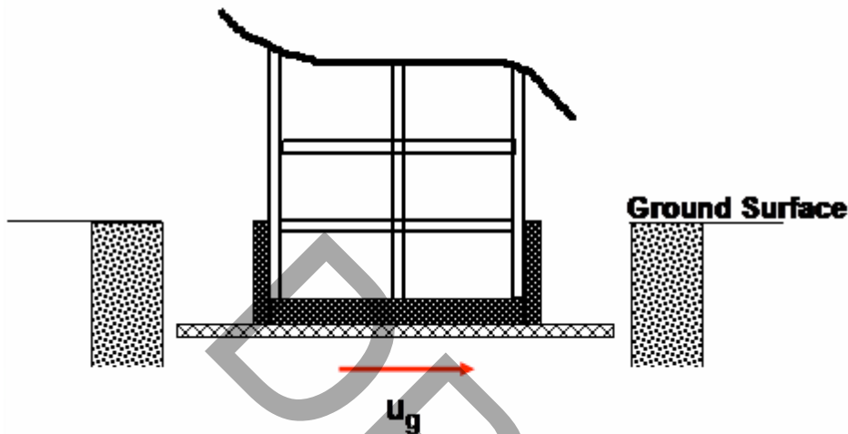
5 6 Figure 7.1 Sketch of simplified model for the building and subterranean levels.
