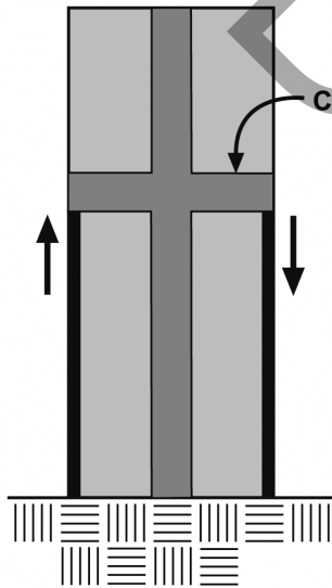
Figure 6.7 Illustration of outriggers used to reduce overturning demands at base of vertical elements of the seismic-force-resisting system.
