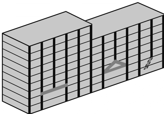
7 Figure 6.4 Illustration of undesirable column transfer and offset conditions.
