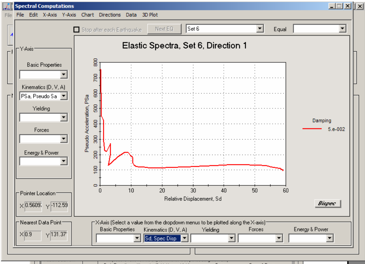
1994 Northridge Sylmar Converter 052 - 3.5 seconds
