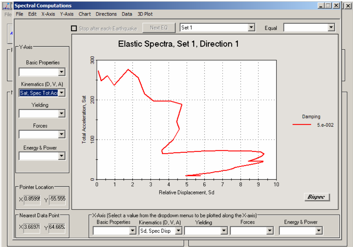
1940 El Centro 180 component – T = 3 seconds
