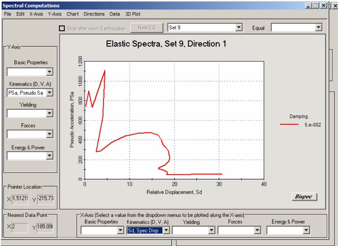
1972 San Fernando Pacoima Dam – 164 – T =5s seoncds
