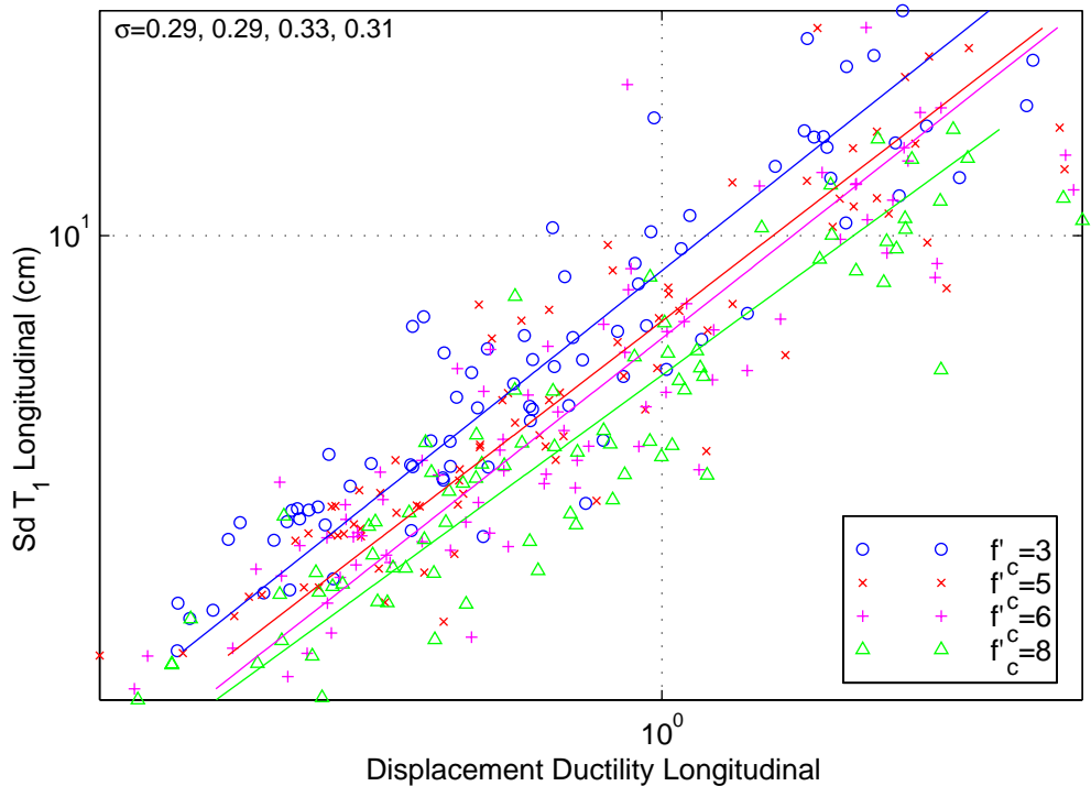
Intensity Measure vs Damage Measure (Parameters)
