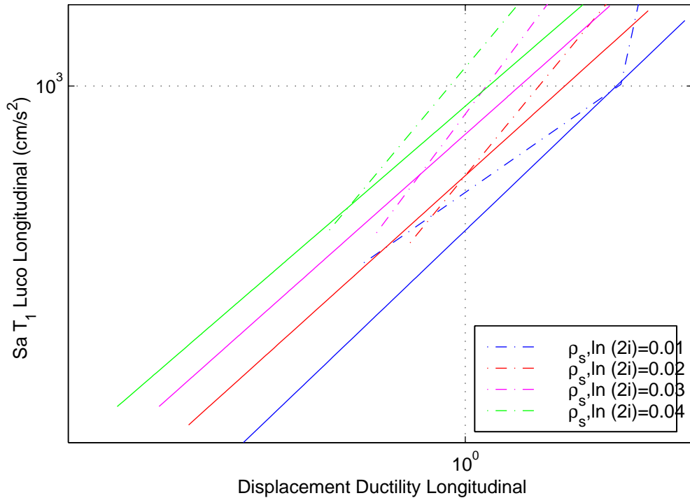
Intensity Measure vs Demand Measure (Parameters) IDA (-.) /PSDM (-)
