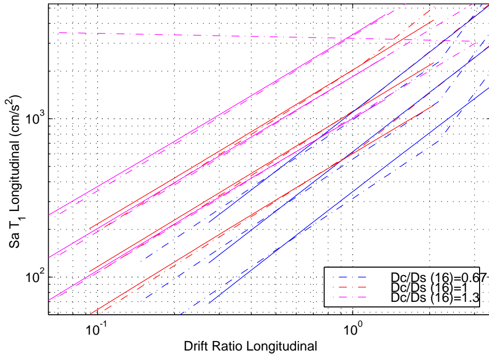
Intensity Measure vs Demand Measure (Parameters) PSDA (-)/IDA (-.)
