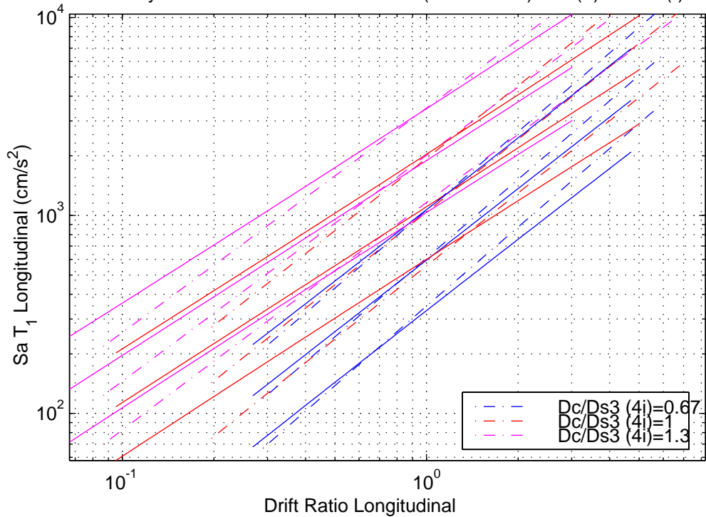
Intensity Measure vs Demand Measure (Parameters) IDA (-.)/PSDM (-)
