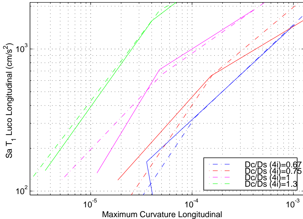
Intensity Measure vs Demand Measure (Parameters) PSDA (-)/IDA (-.)
