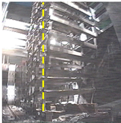
Photo 9. Loss the stability of frame just before collapse
