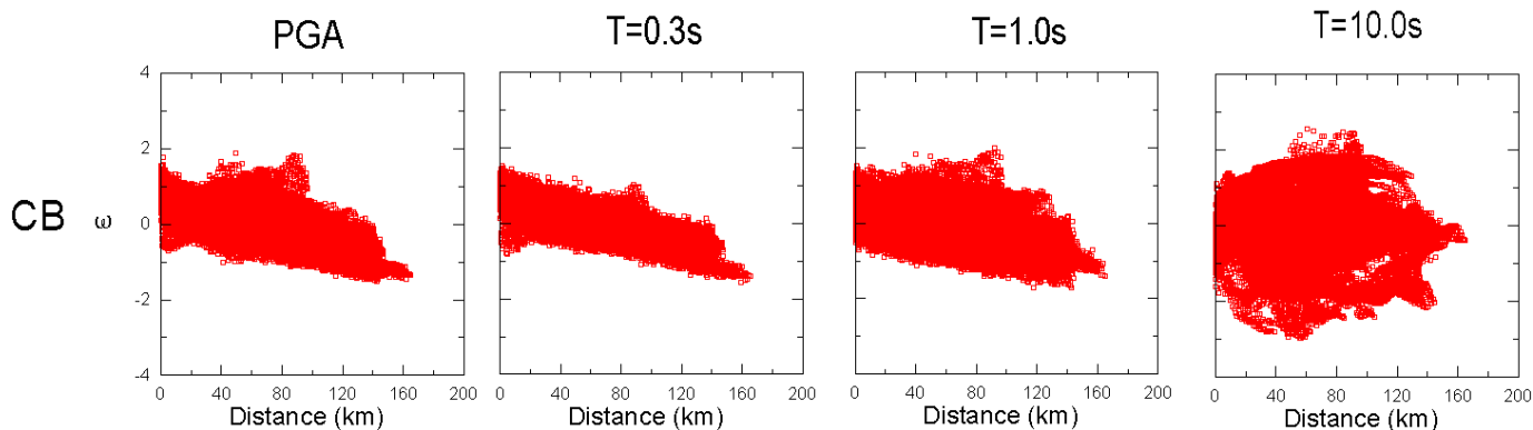
Figure 2: The intra-event residuals of the ShakeOut motions (original southern hypocenter) relative to the CB GMPE for the IMs of PGA and T=0.3s , 1.0, and 10 sec spectral acceleration versus rupture distance.
